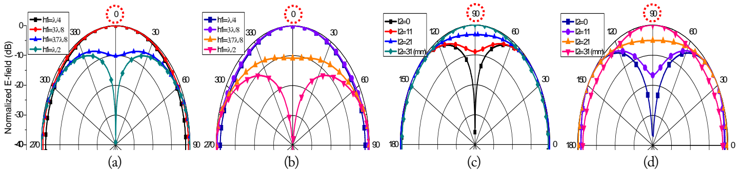
Fig. 6. The predicted radiation pattern using equivalent model of top-hat loaded antenna. (a) Mathematical results according to the variation of height h_1 when l_2 = 31 mm, (b) simulation results according to the variation of height h_1 when l_2 = 31 mm, (c) mathematical results according to the variation of length l_2 when h_1 = 61 mm, and (d) simulation results according to the variation of length l_2 when h_1 = 61 mm.
